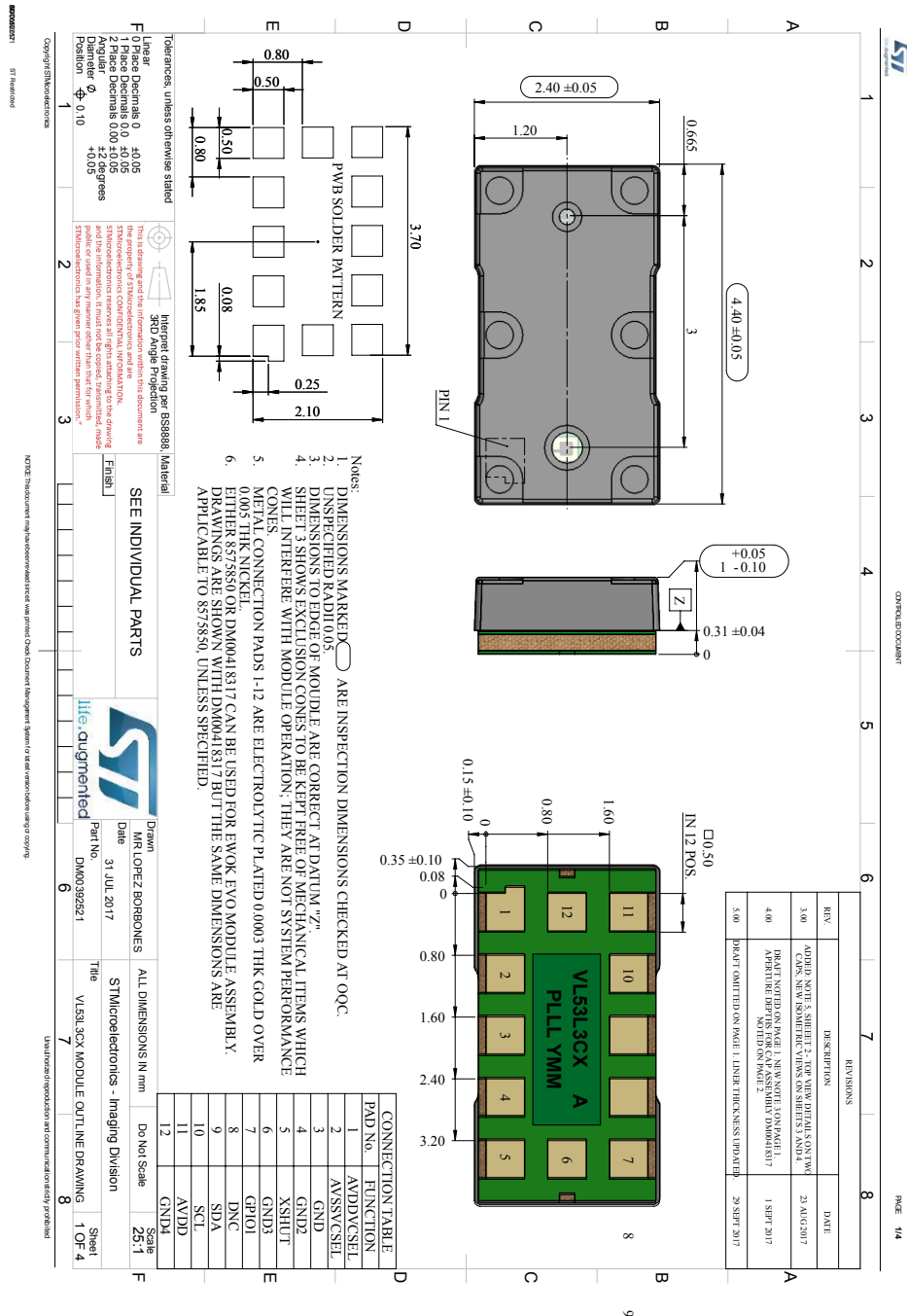
Figure 16. Outline drawing 1/4
